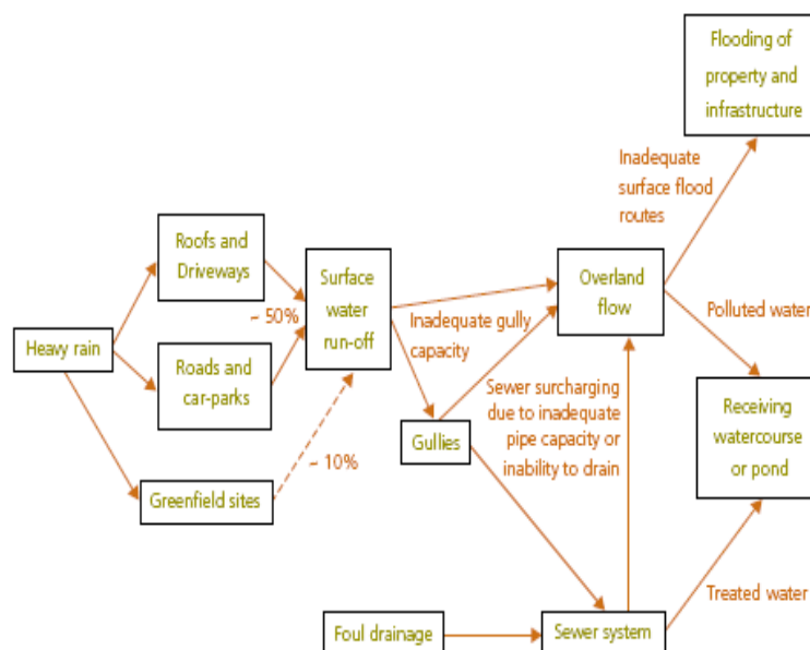
Figure Four: Surface Water Main Flood Routes
