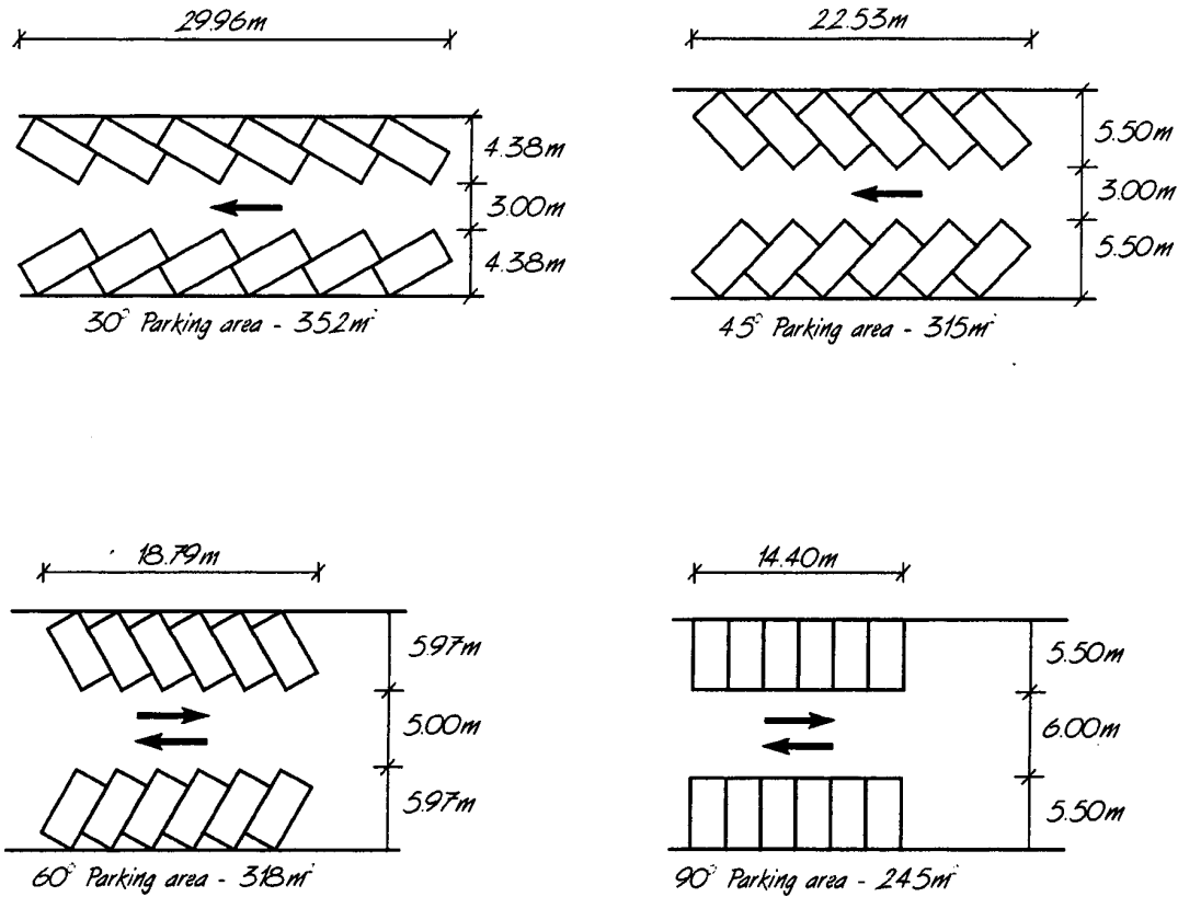
LAYOUT OF PARKING AREAS FOR 12 SPACES OF 5.5m x 2.4m
