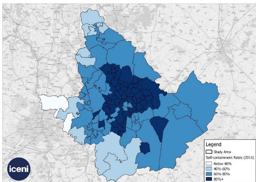
Figure 4.15: Self-Containment Rates, 2011
