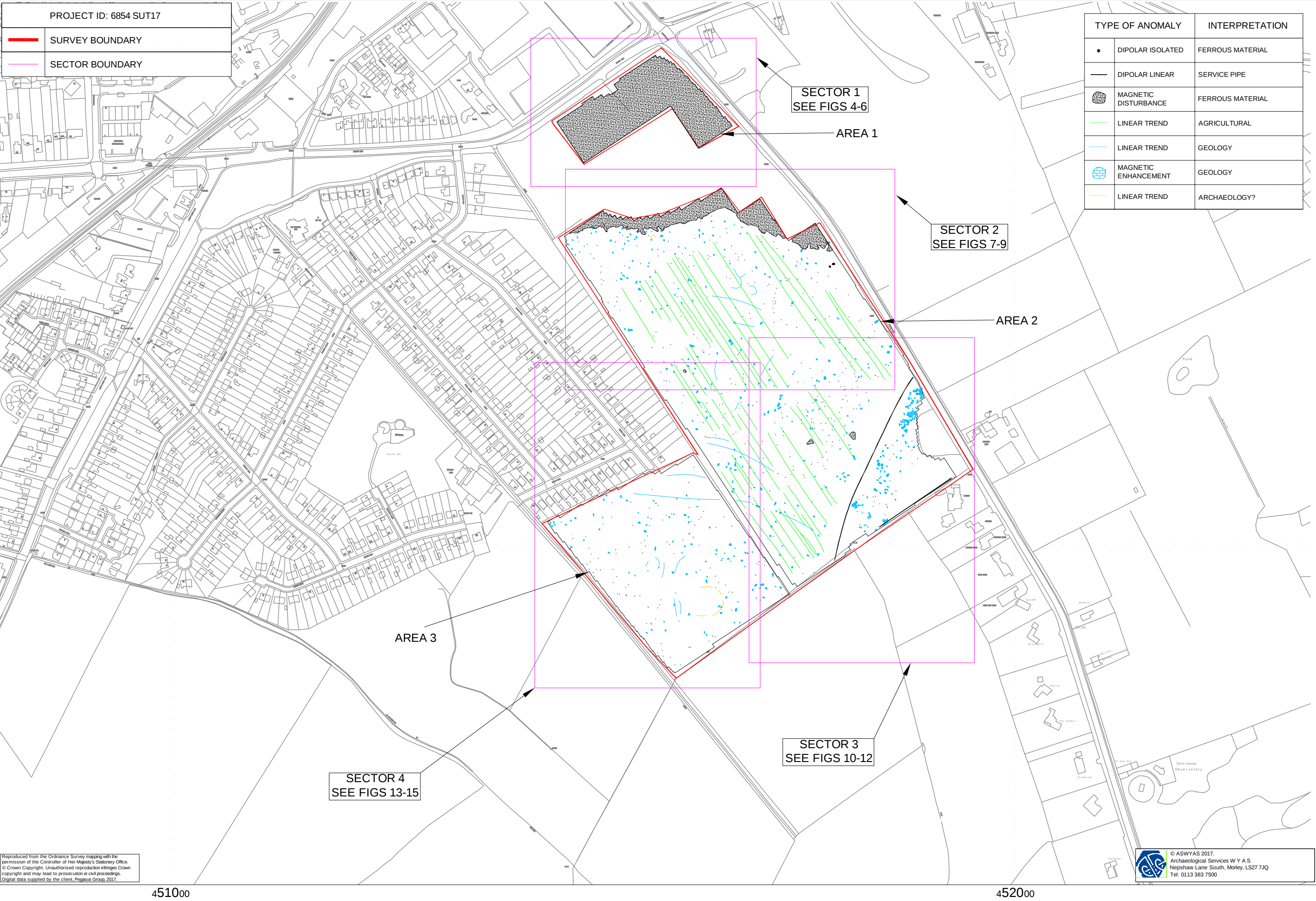
Fig. 3. Overall interpretation of magnetometer data (1:4000 @ A3)
